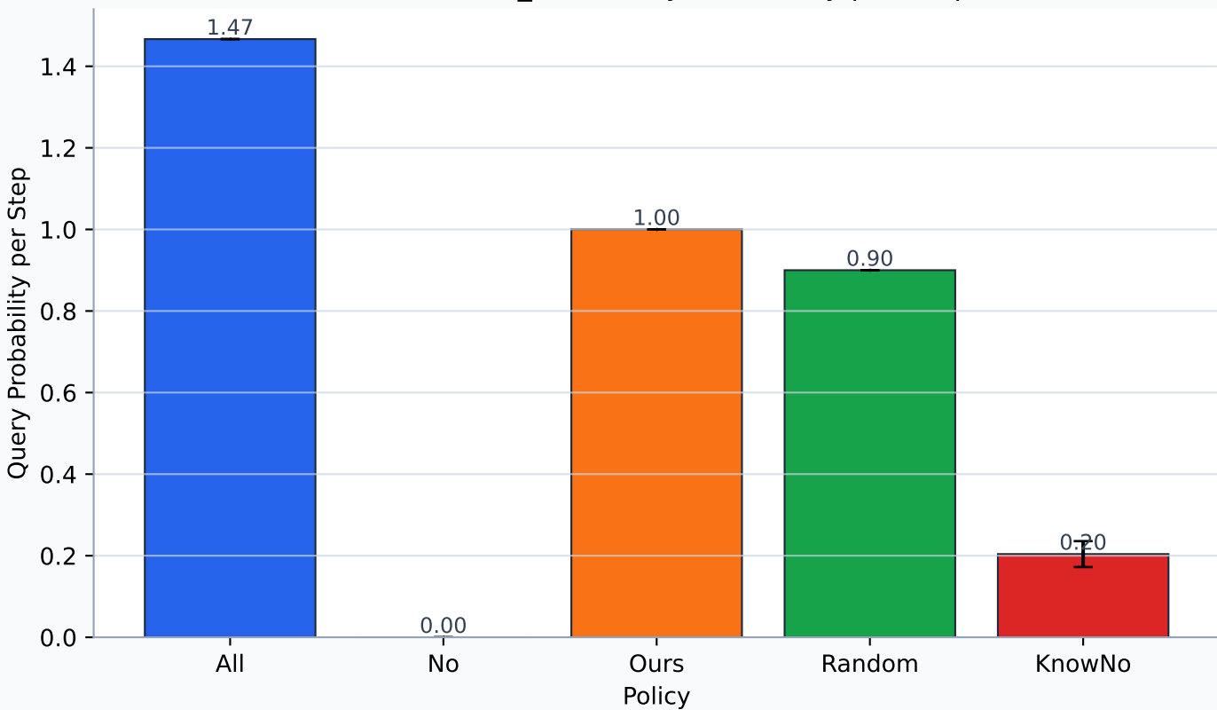
waste scene_01 - Query Probability per Step
