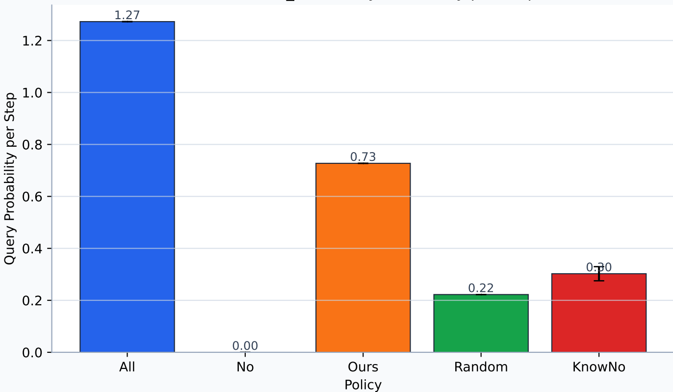
waste scene_03 - Query Probability per Step
