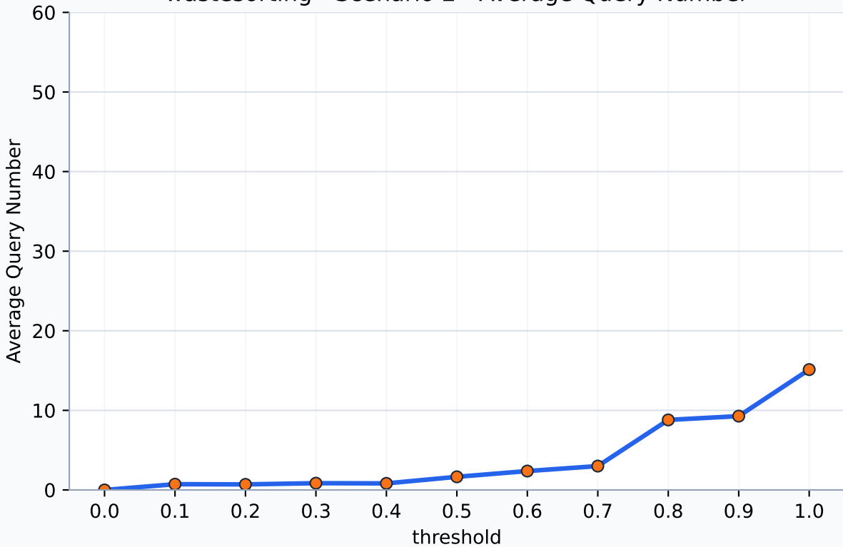
wastesorting - Scenario 2 - Average Query Number
