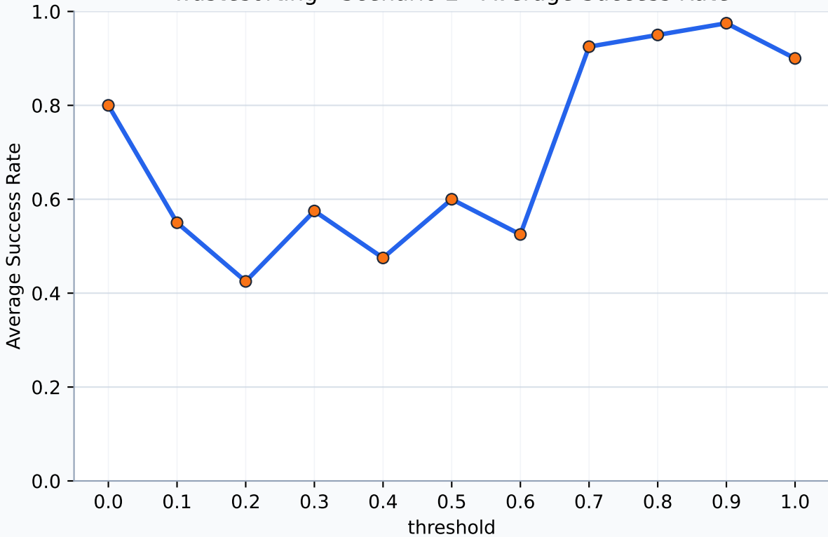
wastesorting - Scenario 2 - Average Success Rate
