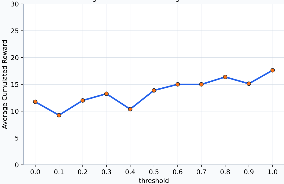
wastesorting - Scenario 3 - Average Cumulated Reward
