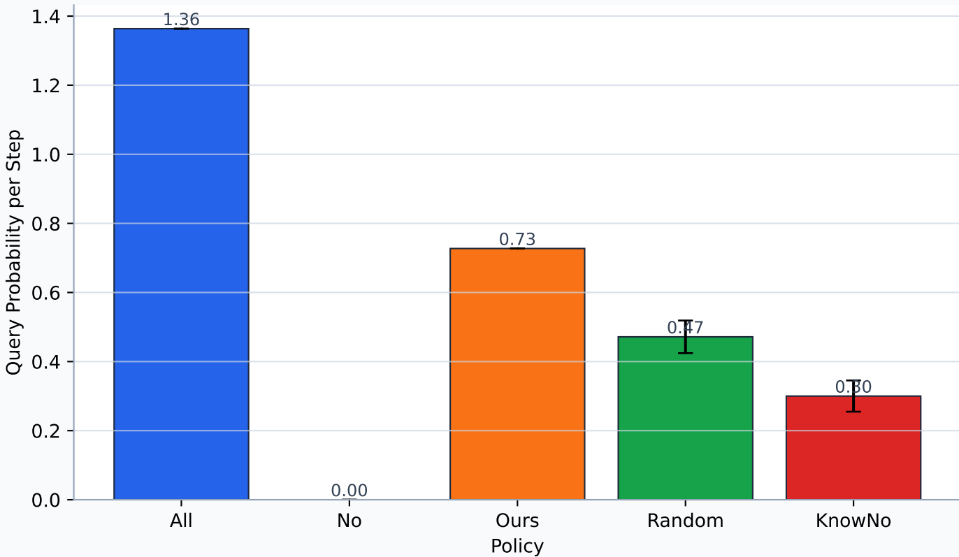
wastesorting scene_02 - Query Probability per Step
