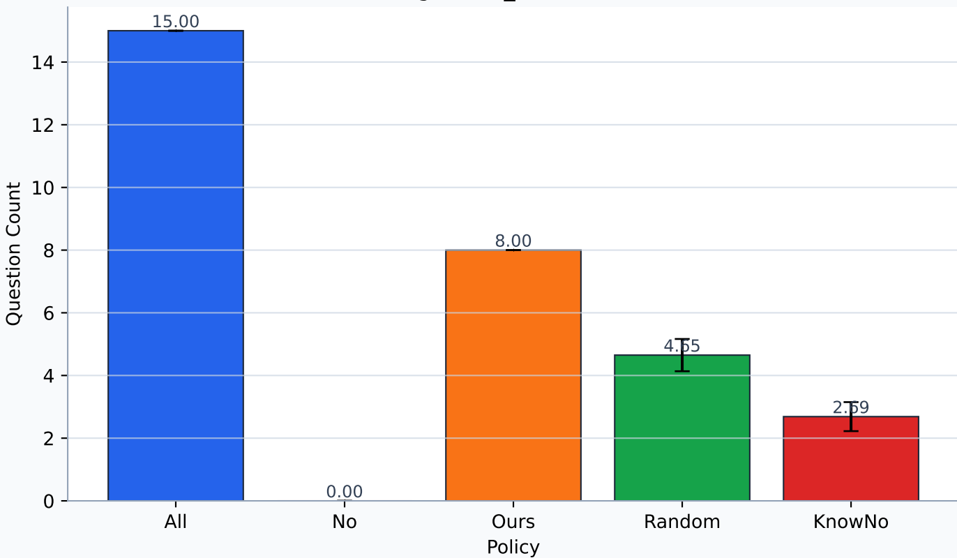
wastesorting scene_02 - Question Count
