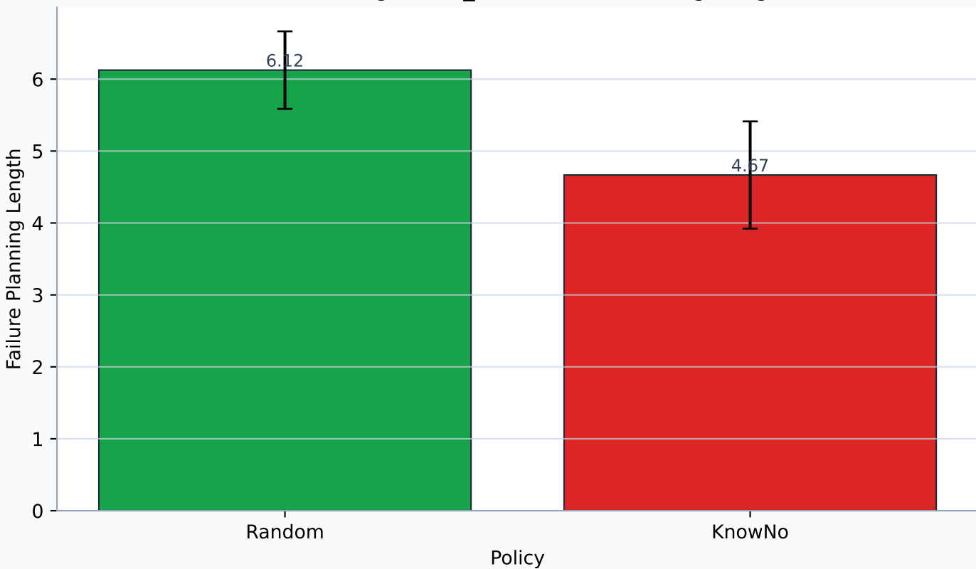
wastesorting scene_03 - Failure Planning Length
