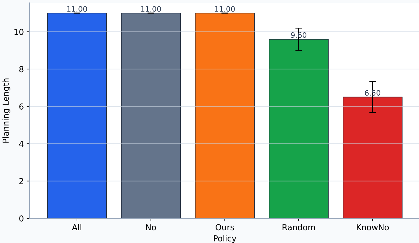
wastesorting scene_03 - Planning Length
