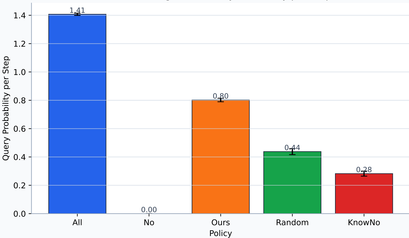
wastesorting total - Query Probability per Step
