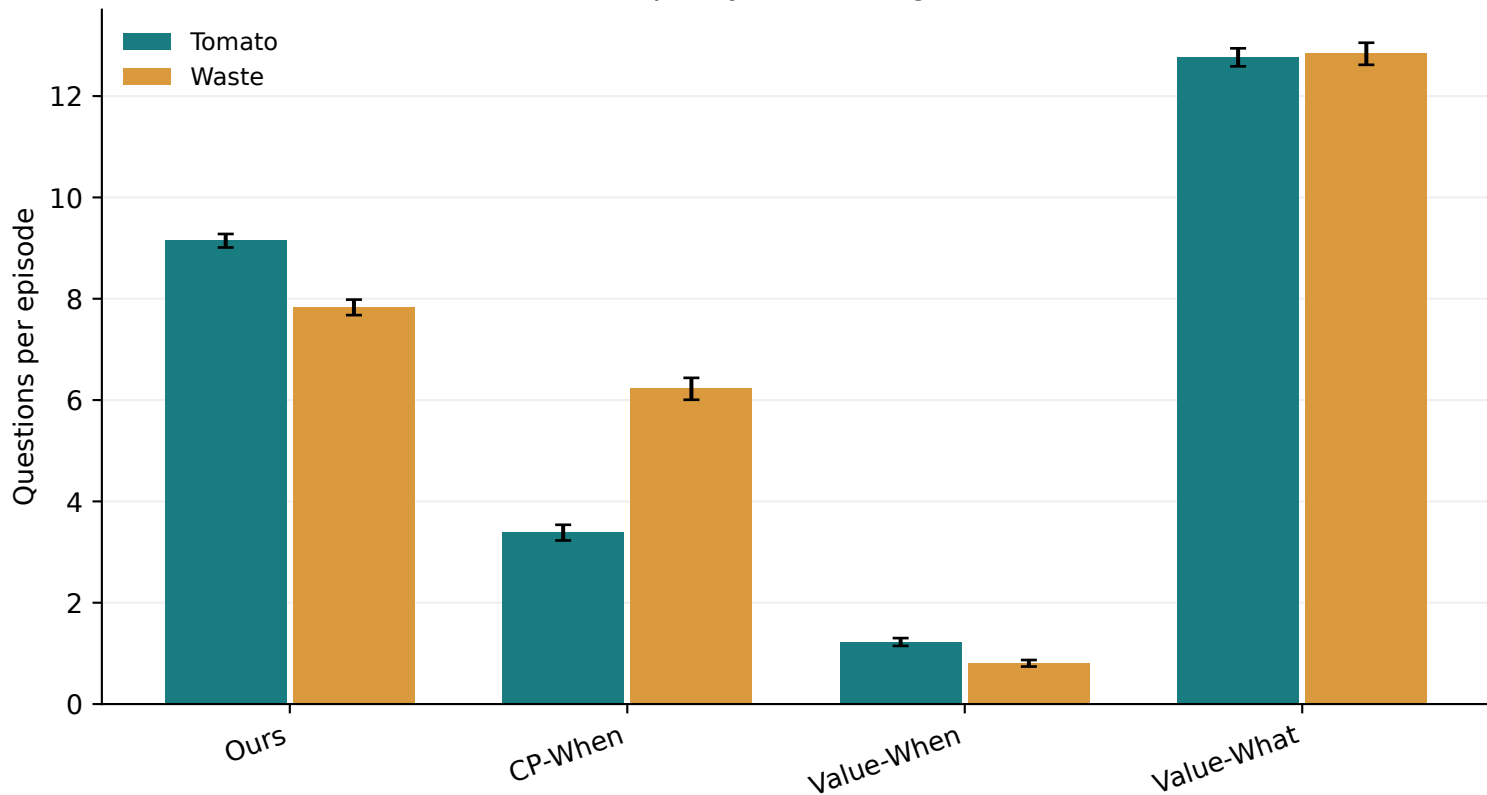
When-What policy ablation (gamma = 0.2)
