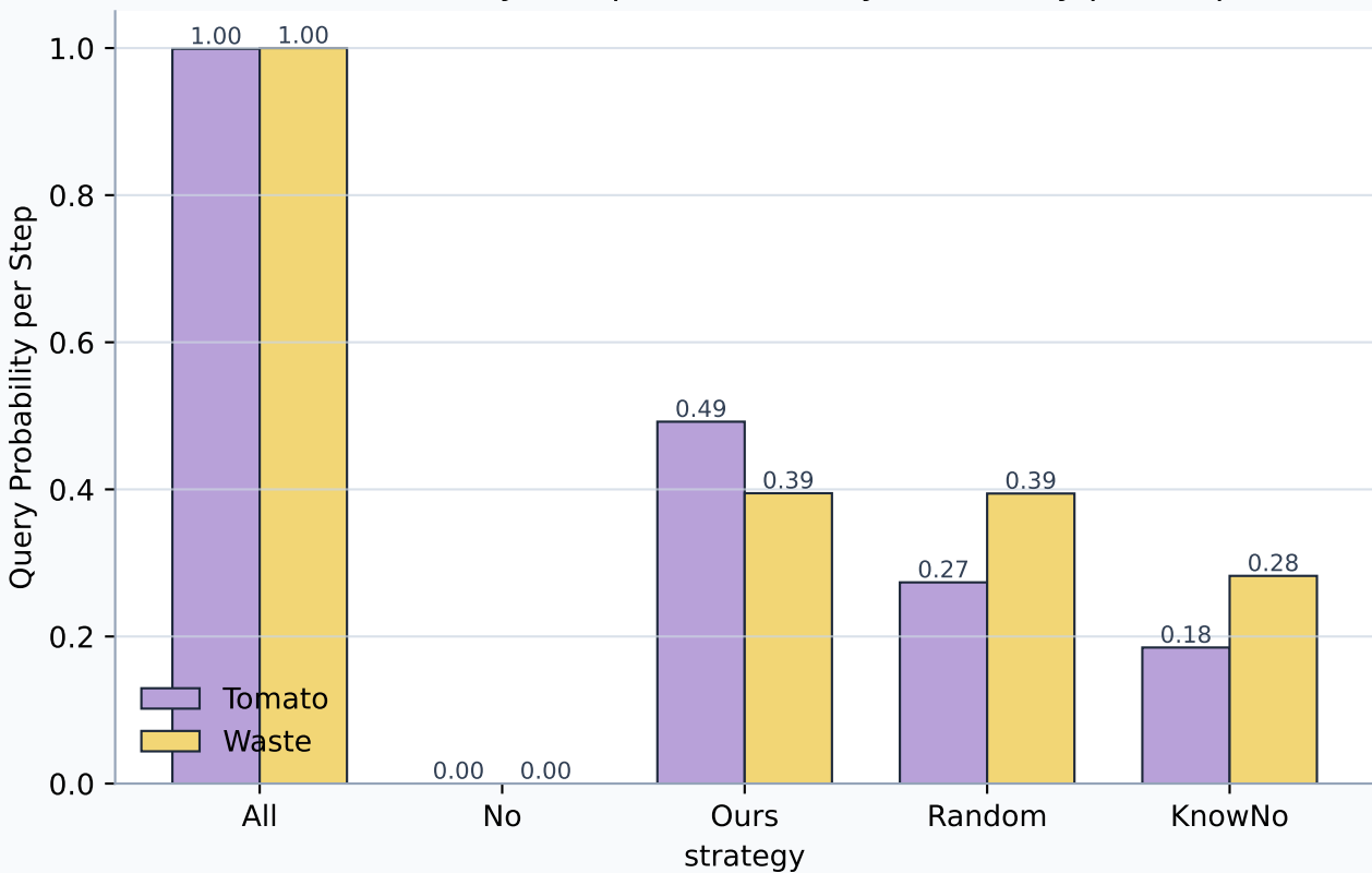
Question Policy Comparison - Query Probability per Step
