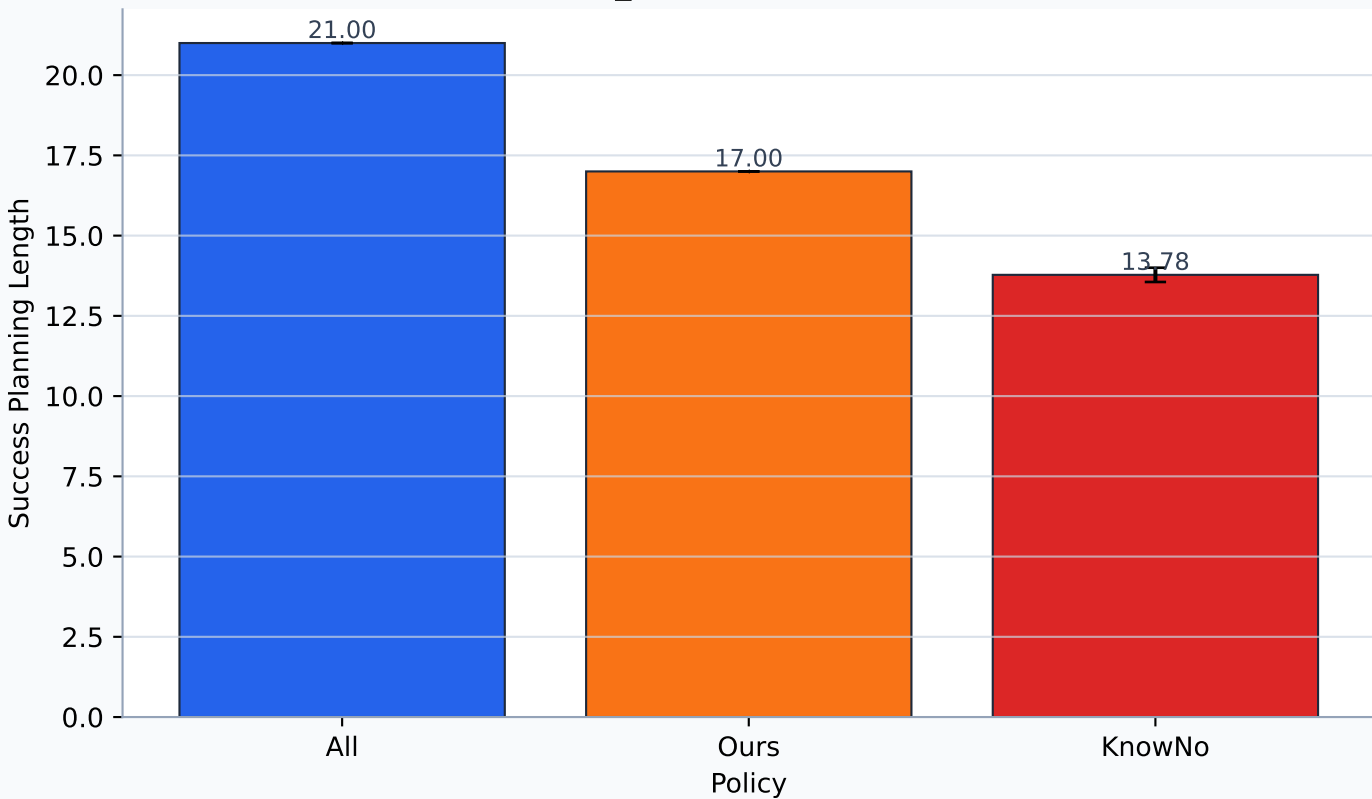
tomato scene_03 - Success Planning Length
