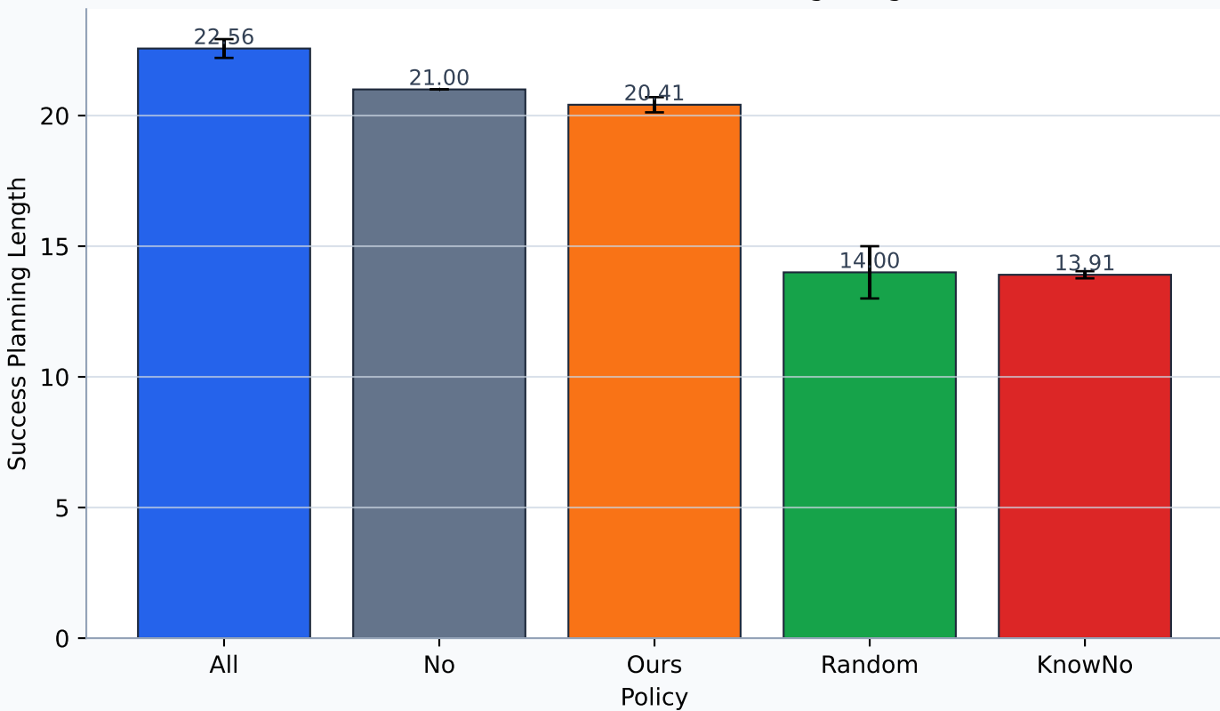
tomato total - Success Planning Length
