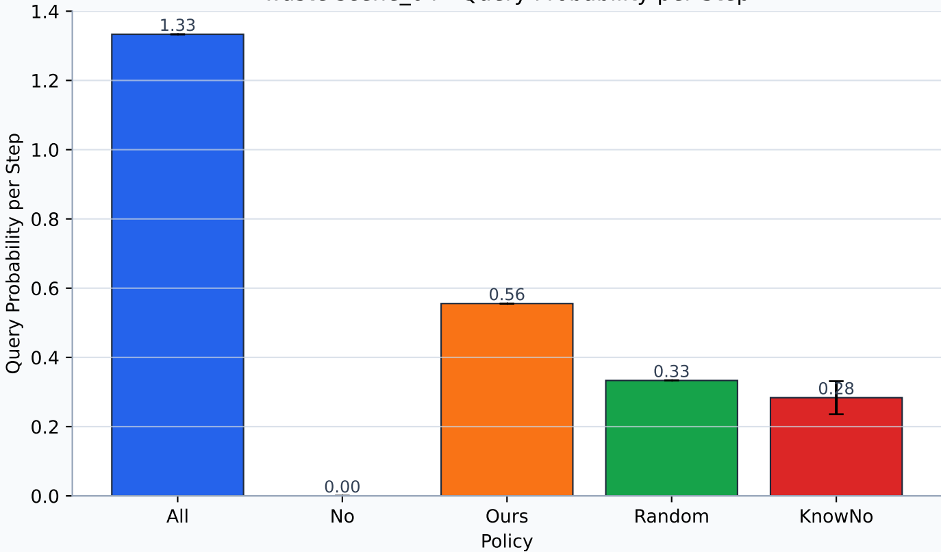
waste scene_04 - Query Probability per Step
