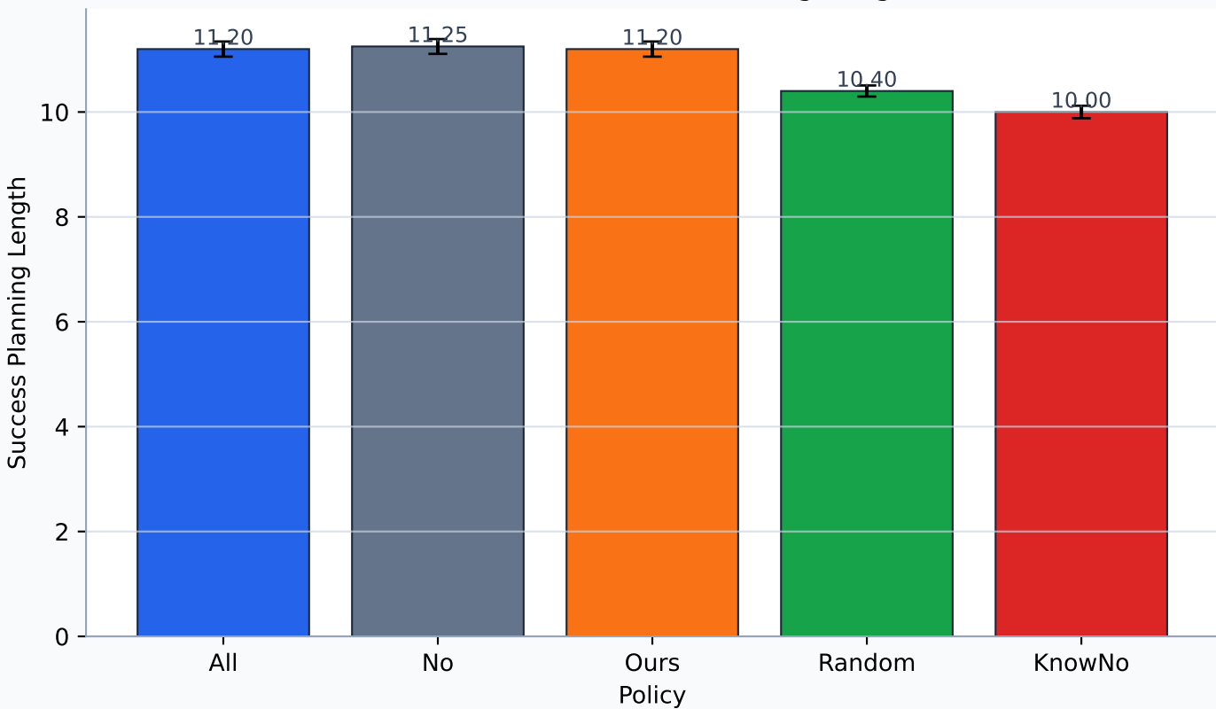
waste total - Success Planning Length
