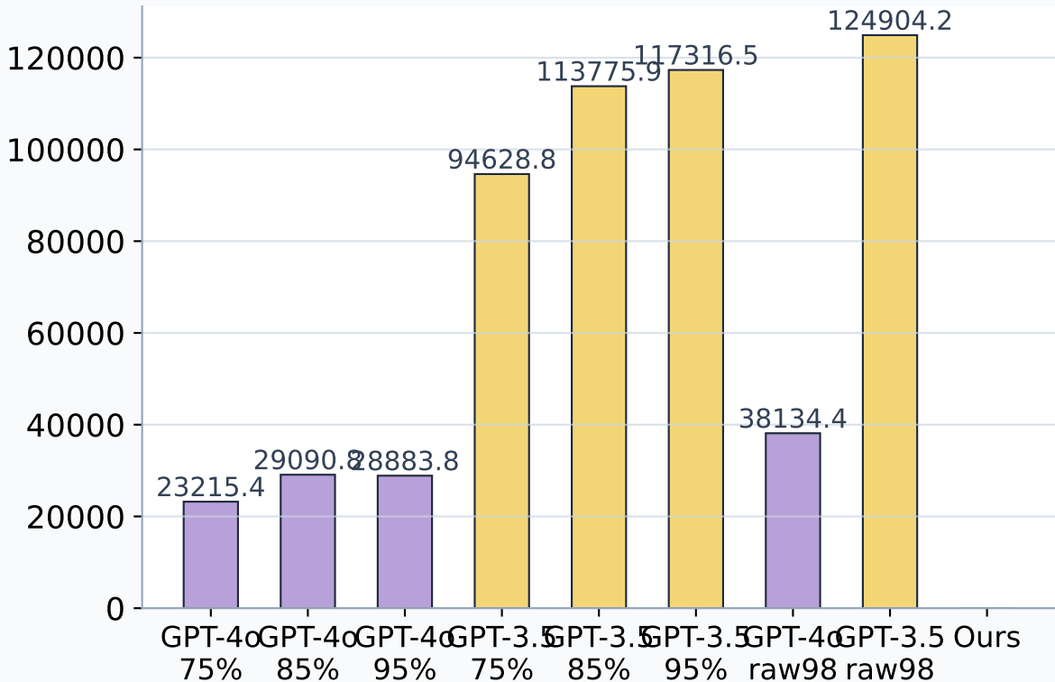
Token Usage
