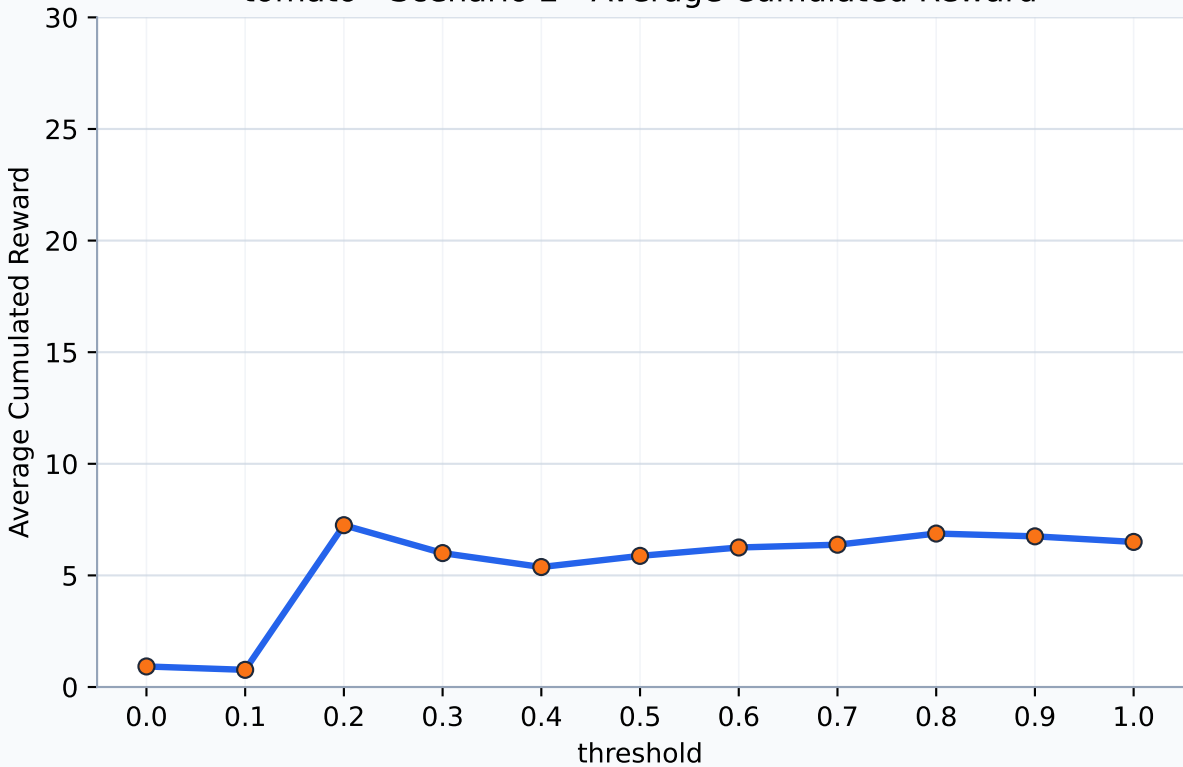
tomato - Scenario 2 - Average Cumulated Reward
