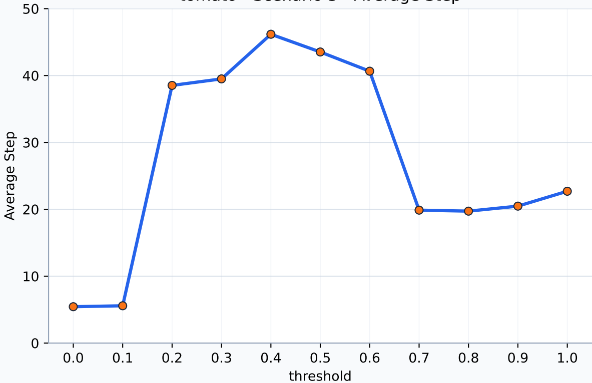
tomato - Scenario 3 - Average Step
