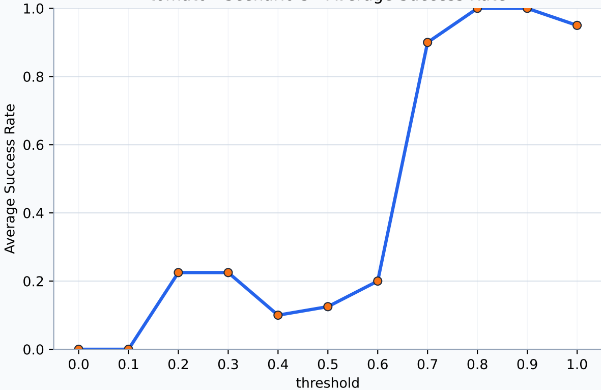
tomato - Scenario 3 - Average Success Rate
