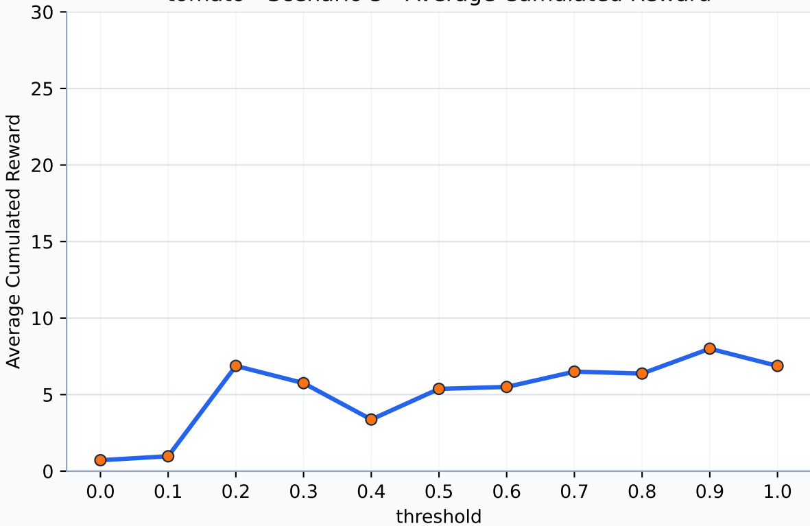
tomato - Scenario 5 - Average Cumulated Reward
