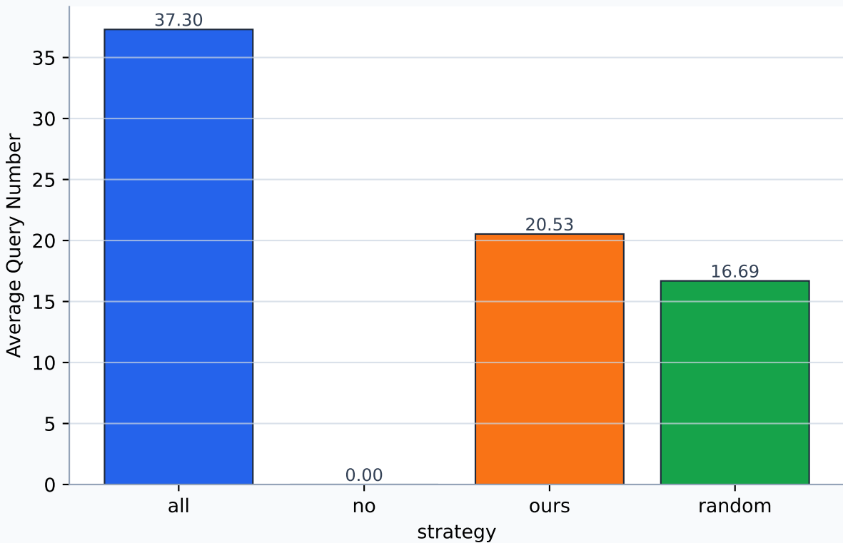
tomato - question policy comparison - Average Query Number
