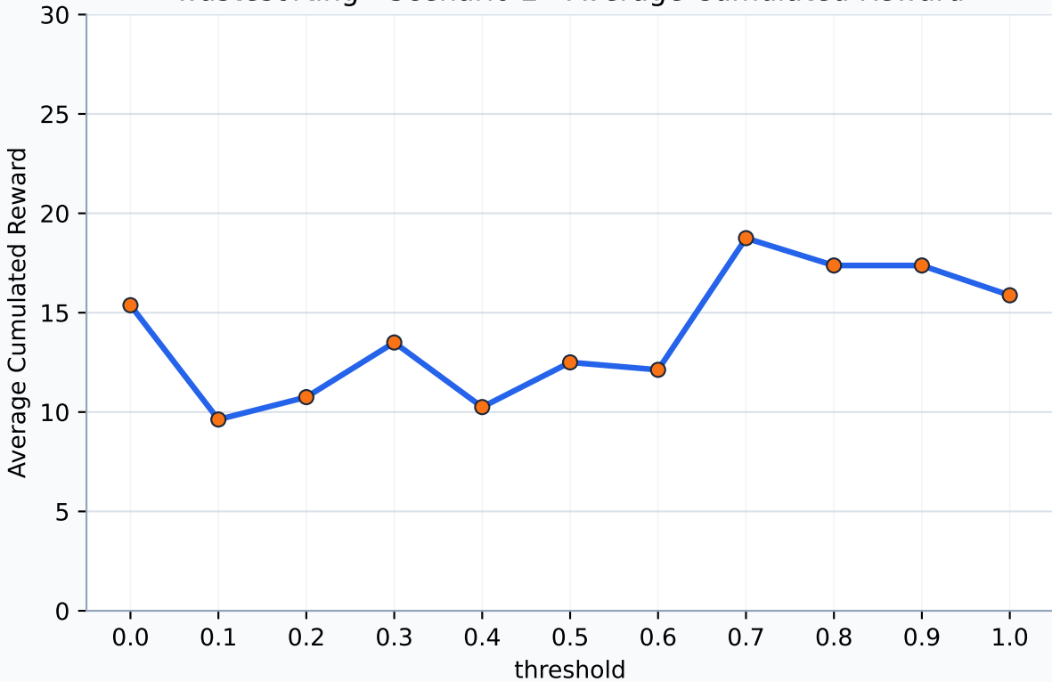
wastesorting - Scenario 2 - Average Cumulated Reward
