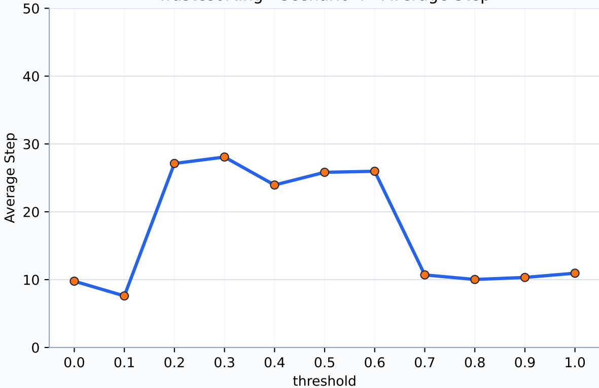
wastesorting - Scenario 4 - Average Step
