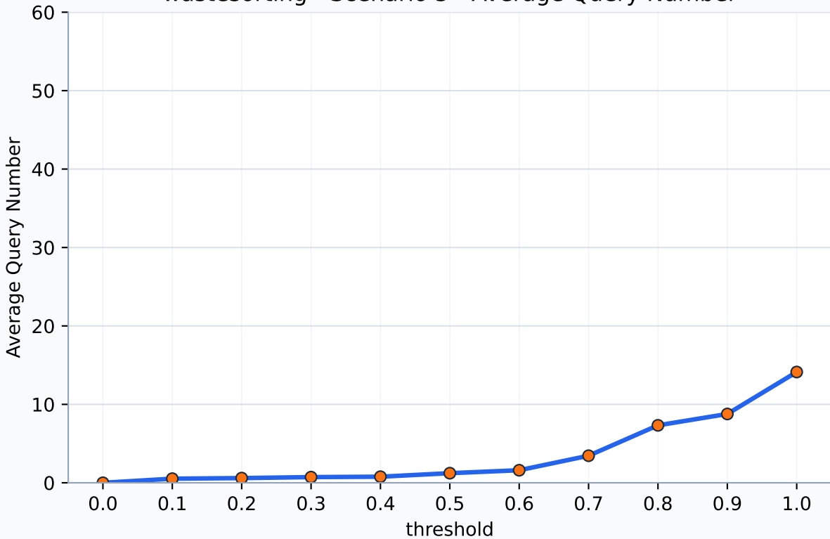
wastesorting - Scenario 5 - Average Query Number
