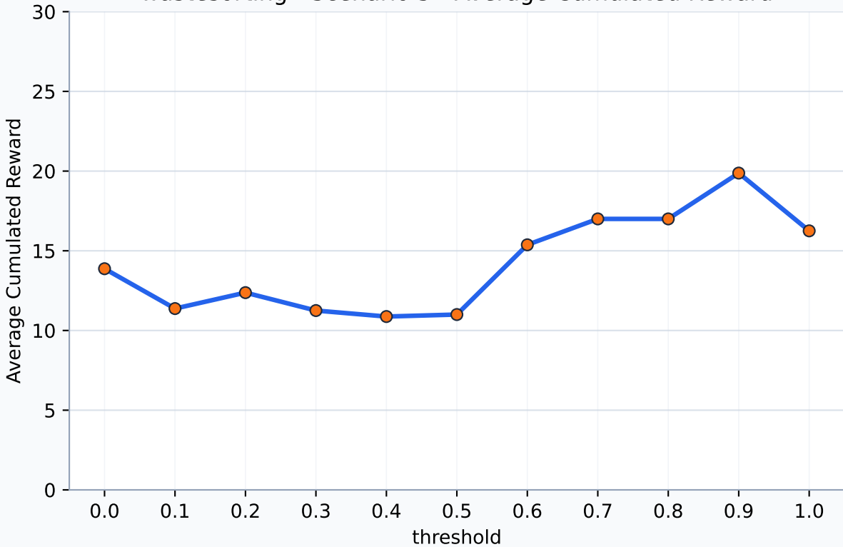
wastesorting - Scenario 5 - Average Cumulated Reward
