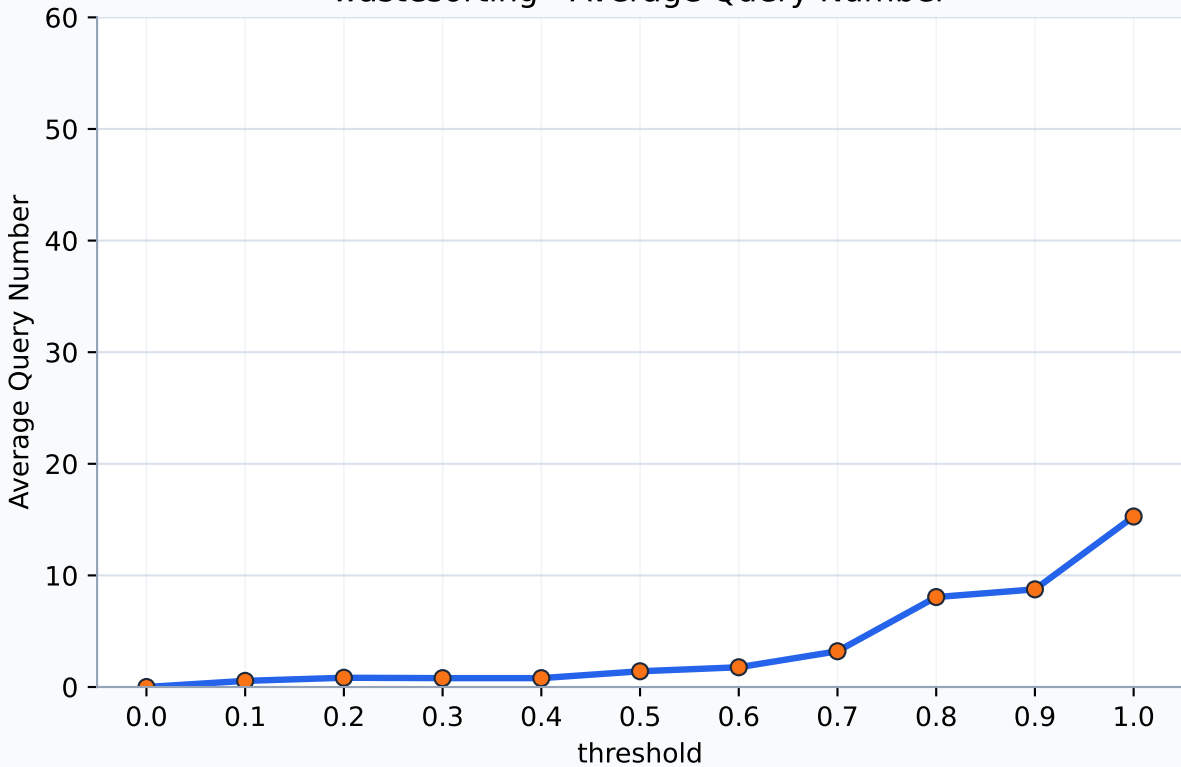
wastesorting - Average Query Number
