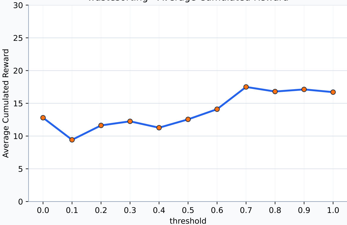
wastesorting - Average Cumulated Reward
