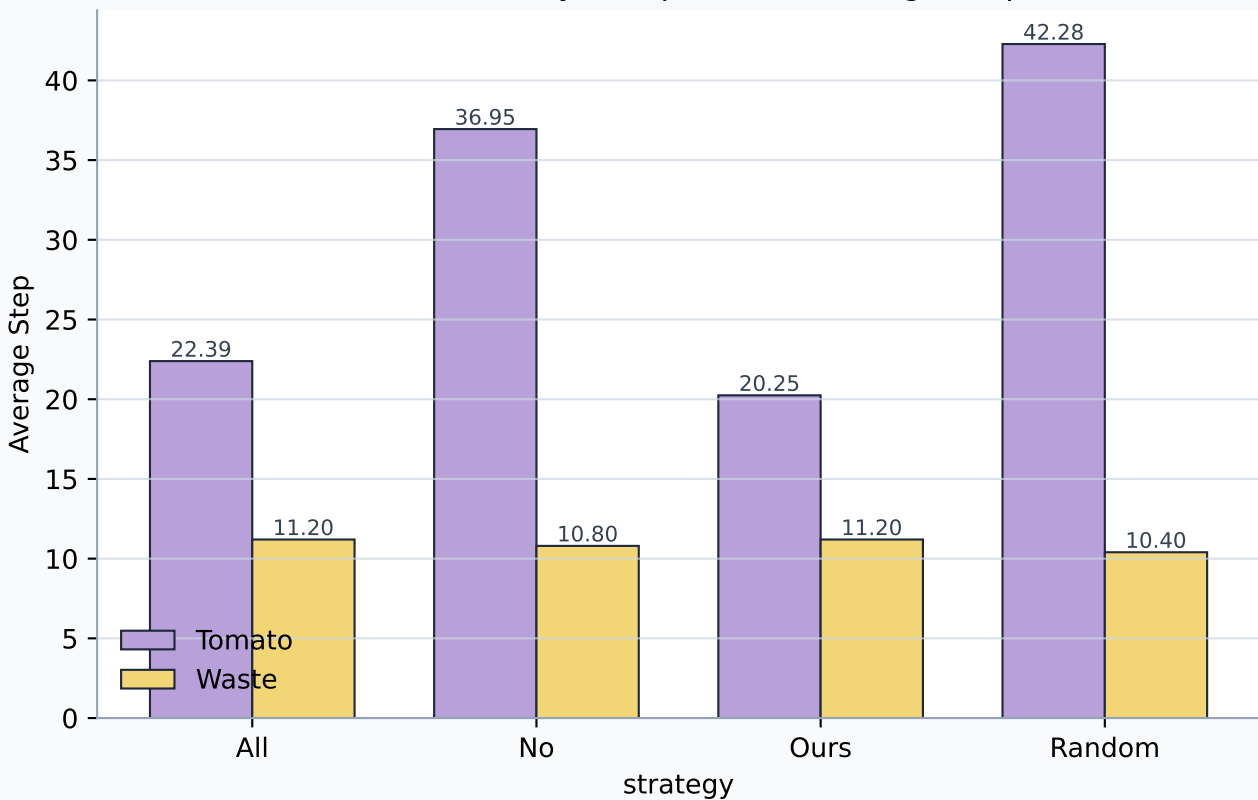
Question Policy Comparison - Average Step
