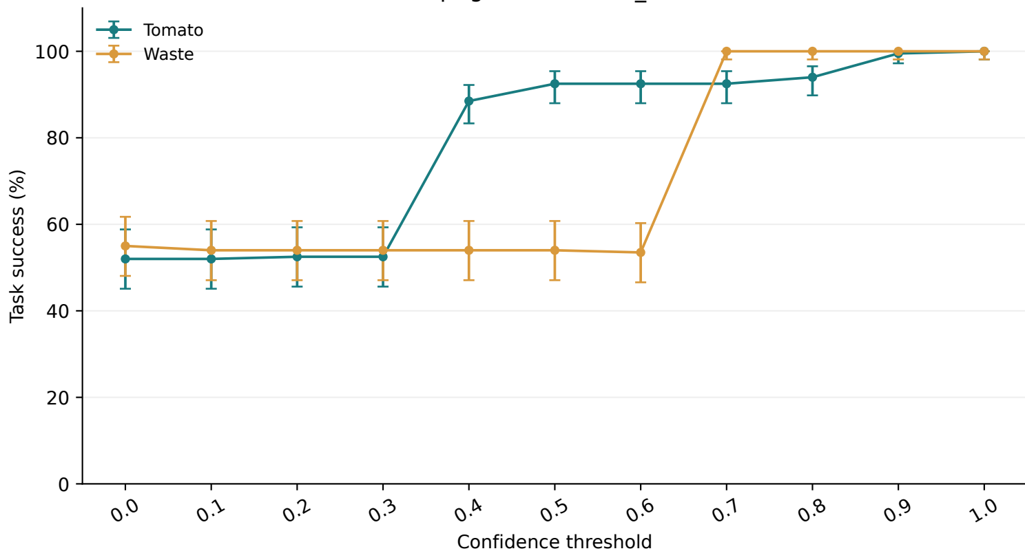
Threshold sweep (gamma=0.2, n_simulations=100)
