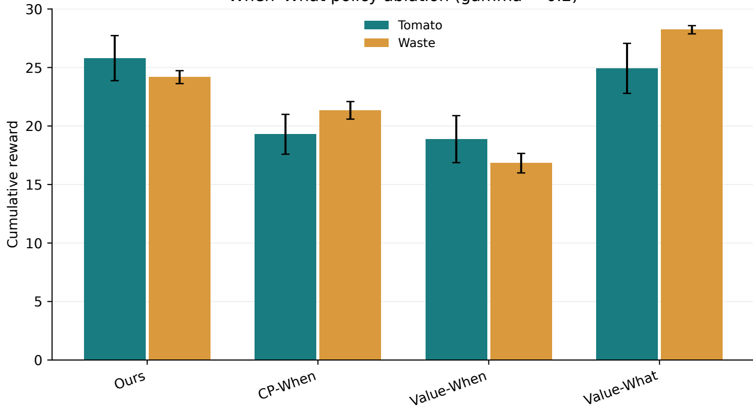
When-What policy ablation (gamma = 0.2)
