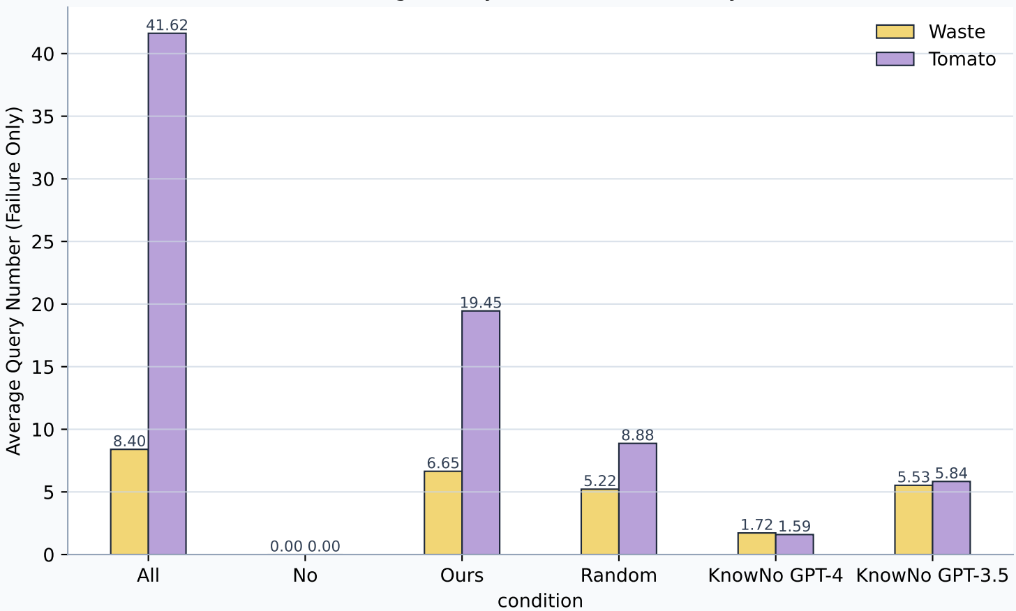
Average Query Number (Failure Only)
