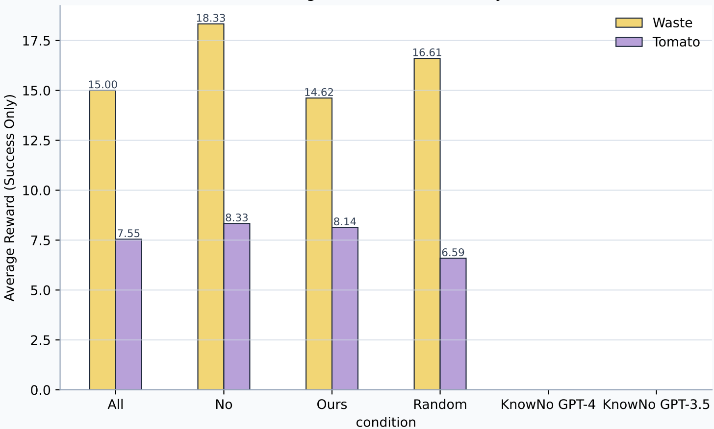
Average Reward (Success Only)
