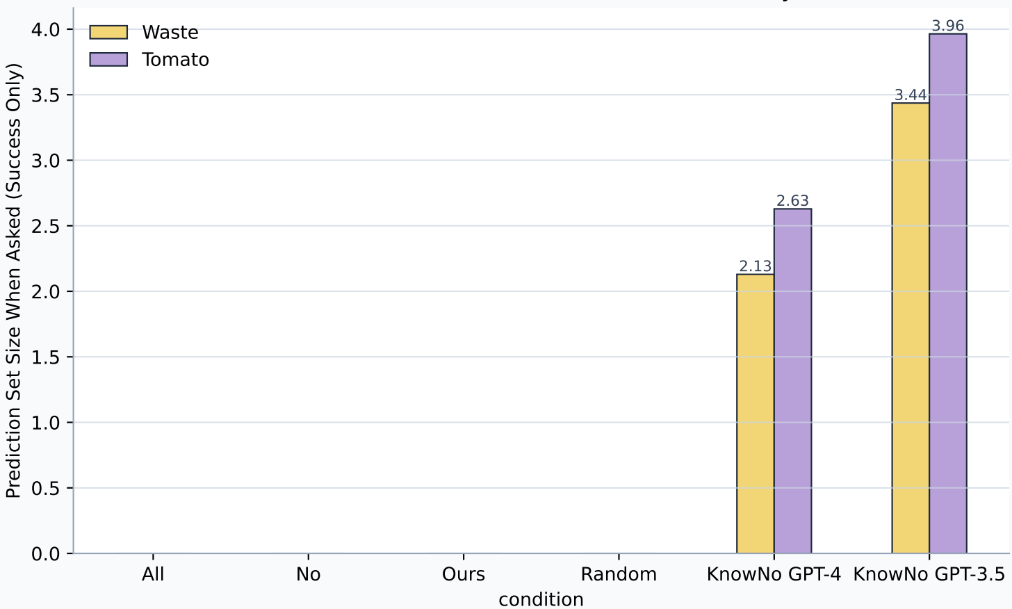
Prediction Set Size When Asked (Success Only)
