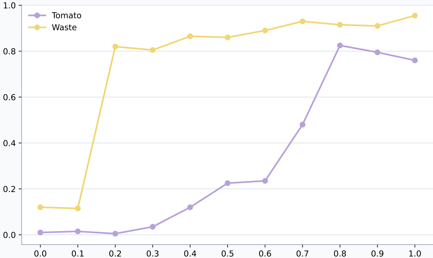
Success Rate
