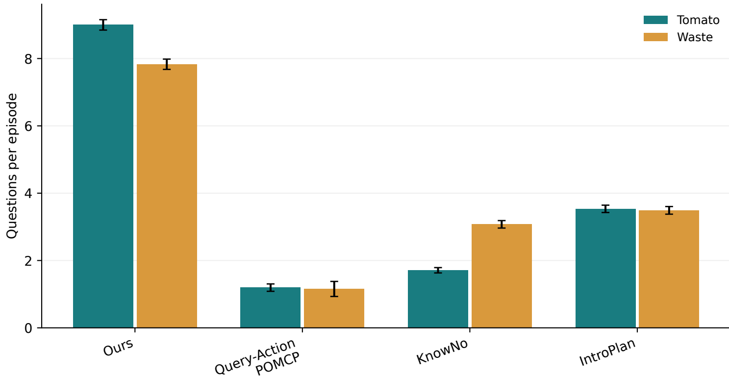
Query baseline comparison
