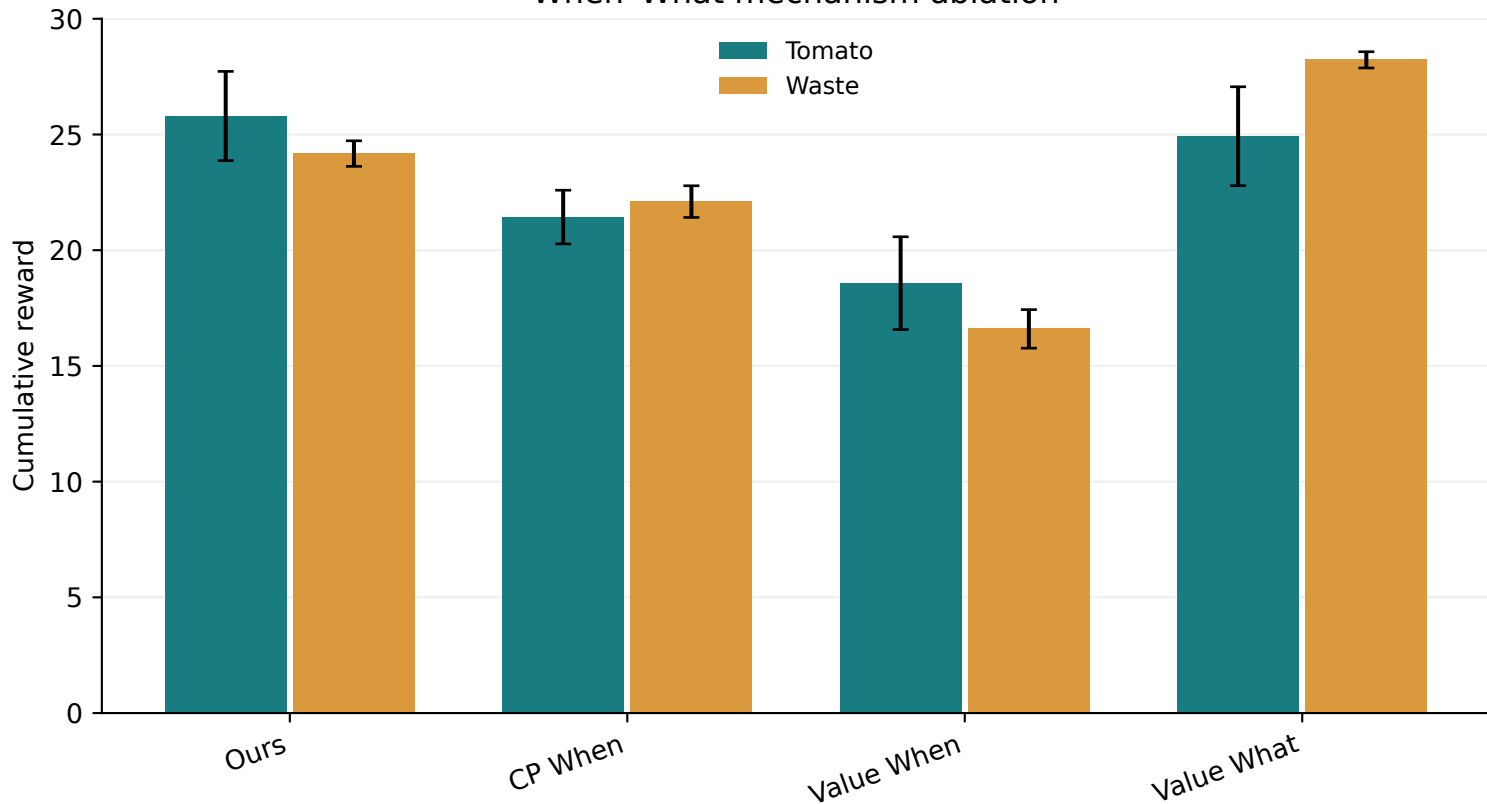
When-What mechanism ablation
