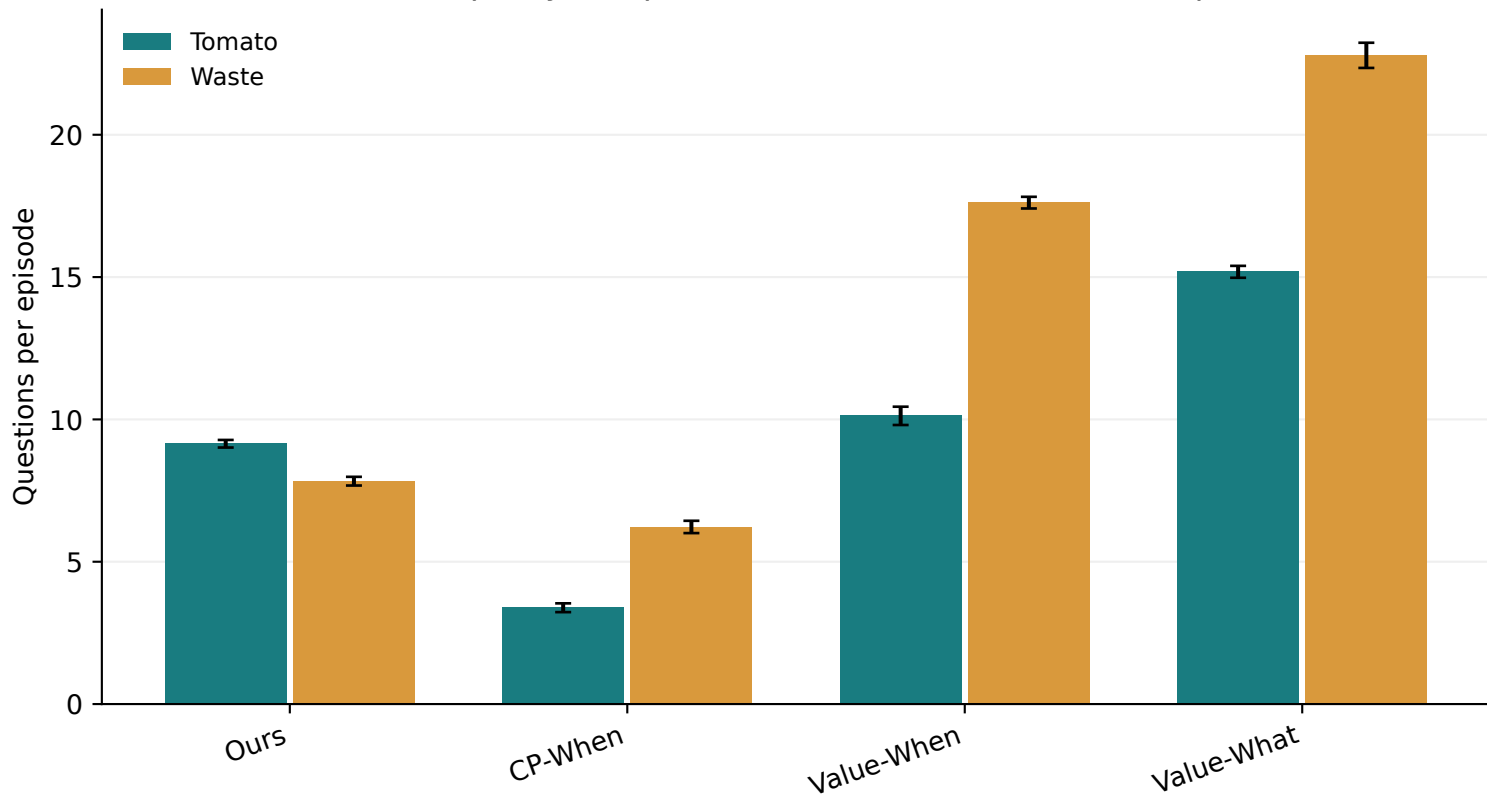
When-What policy comparison (Value-When threshold-loop rerun)
