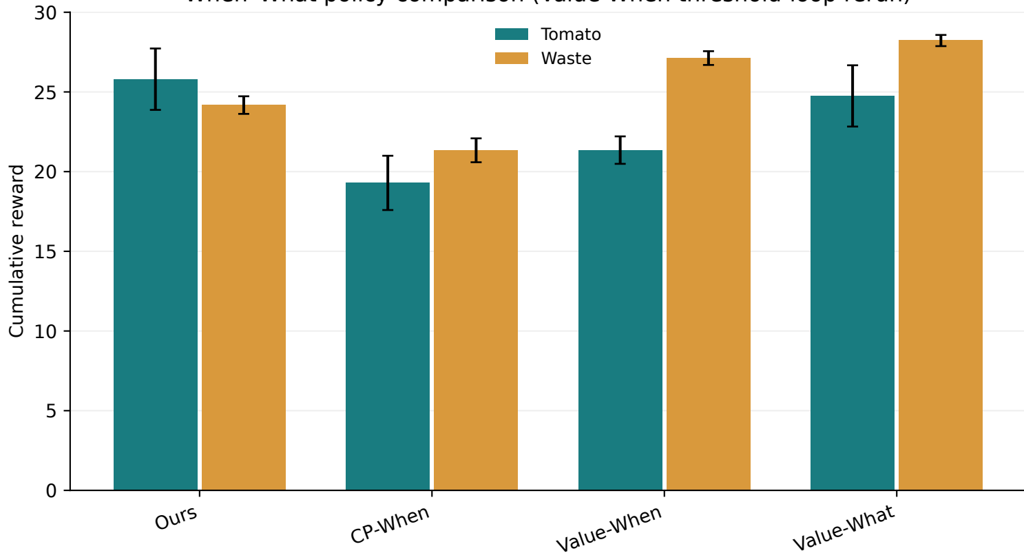
When-What policy comparison (Value-When threshold-loop rerun)
