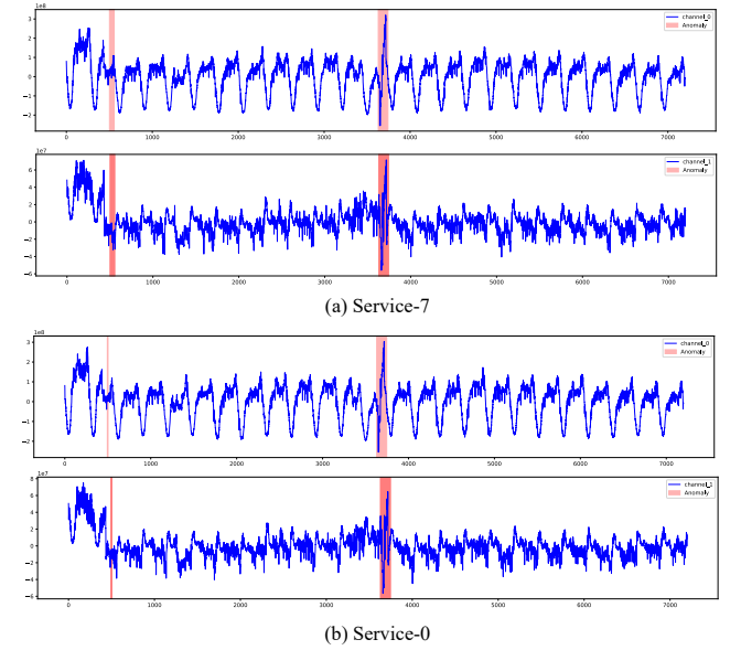
Figure 6: The visualization of SMD data after dimensionality reduction using PCA. (a) and (b) are collected from Service-7 and Service-0 in the SMD dataset respectively.
