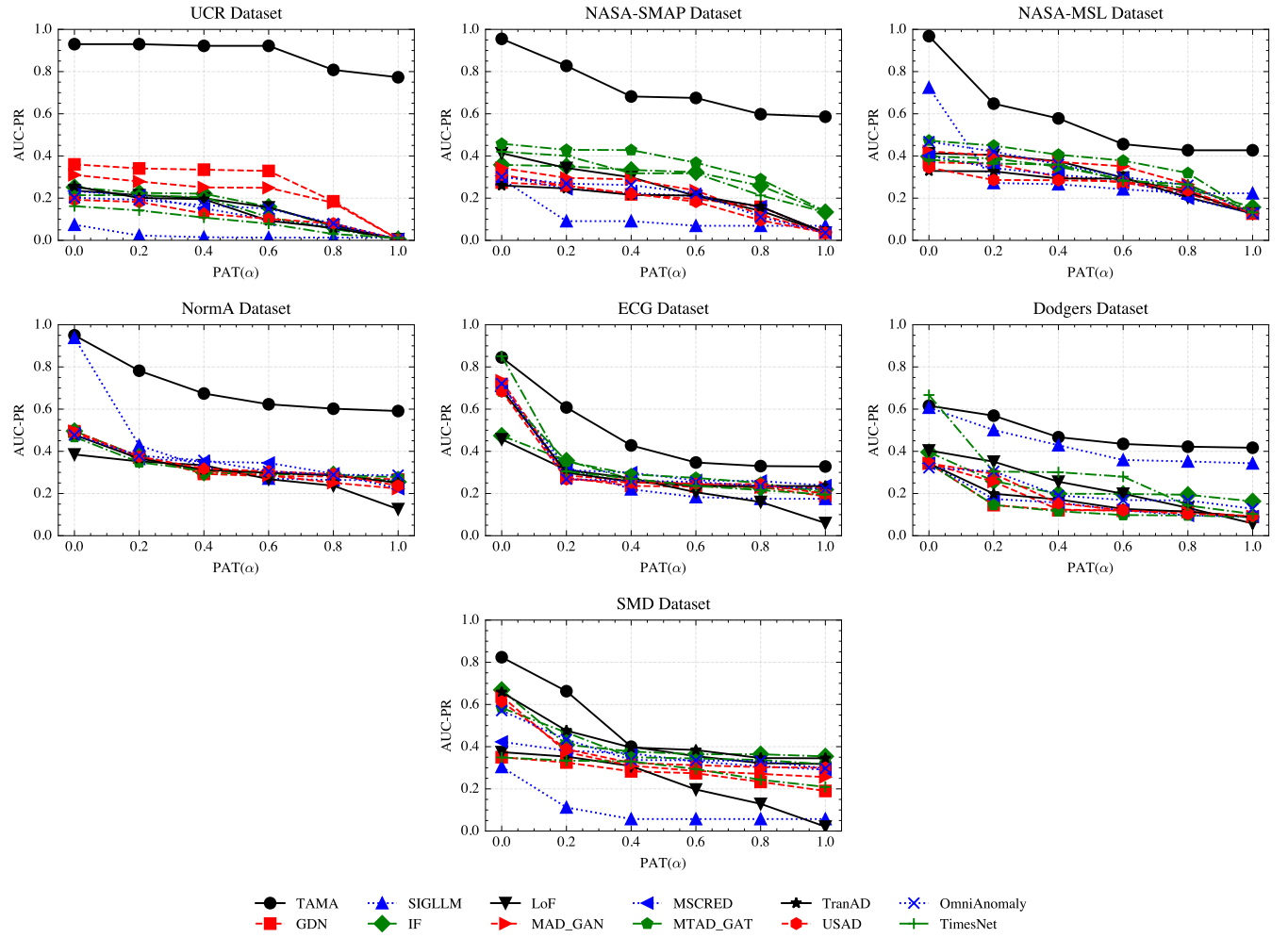
Figure 7: The full AUC-PR results of all models across all datasets at various point-adjustment threshold \alpha (PAT, see Appendix A.2).
