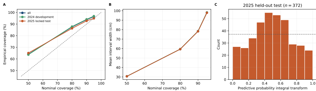
Figure S3: Empirical coverage and interval width for the unit-consistent predictive distribution. Parameters were estimated from the 2024 development cohort; the newly planted, subject-disjoint 2025 cohort was held out. The diagonal in the coverage panel marks exact nominal coverage. Points above the diagonal indicate conservative intervals.
