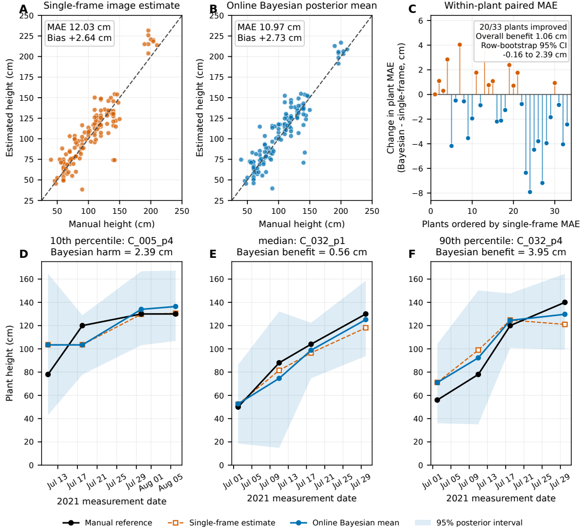
Figure 3: Independent 2021 manual-reference validation. (a,b) Single-frame and Bayesian estimates against manual height for all 132 records; dashed lines mark equality. (c) Within-plant difference in mean absolute error, ordered by single-frame error; negative values favor the Bayesian estimate. (d-f) Trajectories selected by the fixed 10th-, 50th-, and 90th-percentile rule on within-plant benefit, illustrating harm, median behavior, and benefit without residual-based exclusion. Shading is the 95% latent-height posterior interval. Within-record uncertainty is the stationary-camera-row bootstrap interval in panel c and Table 2.
