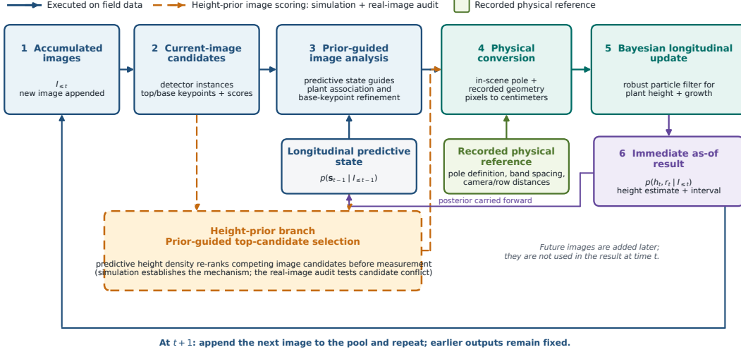
Figure 4: Workflow for the as-of image update. The feedback arrows place prior information inside current-image analysis: the running position state guides detection association and base refinement, and the dashed amber branch uses the predicted height distribution to choose among alternative top candidates. Solid blue stages were executed in the field pipeline; the height-candidate branch was evaluated in controlled simulation and the matched real-image audit. At time t , only I_{\leq t} is available; with settings fixed, a later image starts a new update and does not alter an earlier output.
