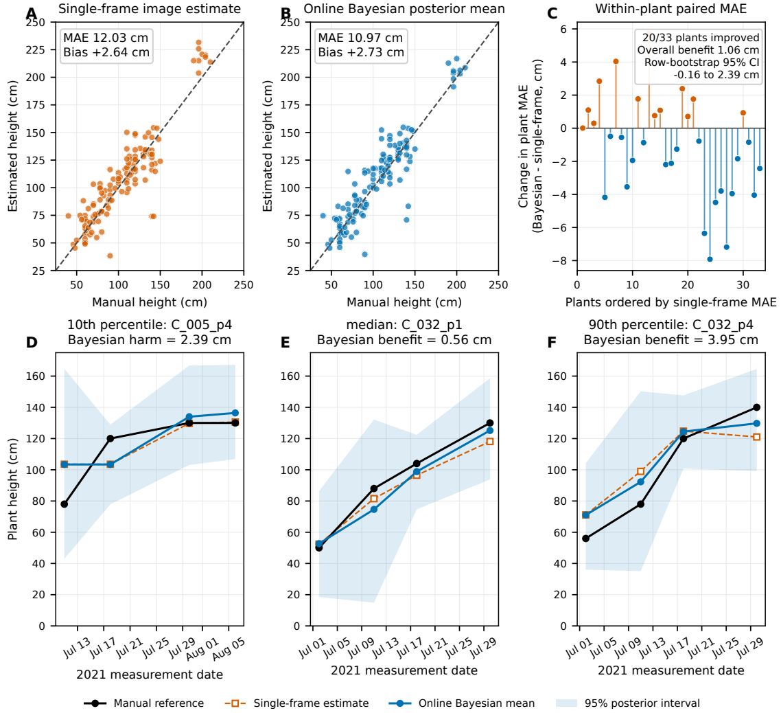
Figure 3: Primary 2021 manual-reference validation. (a,b) Single-frame and Bayesian estimates against manual height for all 132 records; dashed lines mark equality. (c) Within-plant difference in mean absolute error, ordered by single-frame error; negative values favor the Bayesian estimate. (d-f) Trajectories selected by the fixed 10th-, 50th-, and 90th-percentile rule on within-plant benefit, illustrating harm, median behavior, and benefit without residual-based exclusion. Shading is the 95% latent-height posterior interval. The paired uncertainty is the stationary-camera-row bootstrap interval reported in panel c and Table 2.
