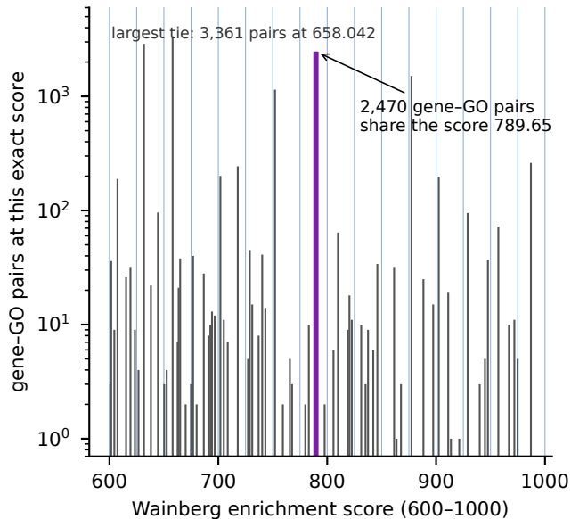
A Enrichment scores are heavily tied
