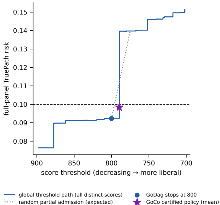
B The 800→775 step overshoots \alpha
