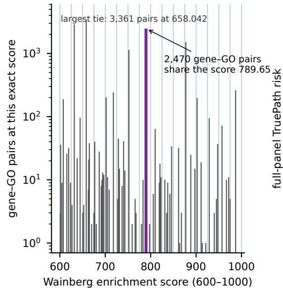
A Enrichment scores are heavily tied
