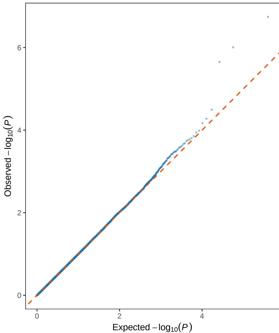
QQ Plot ( \lambda=0.989 )
