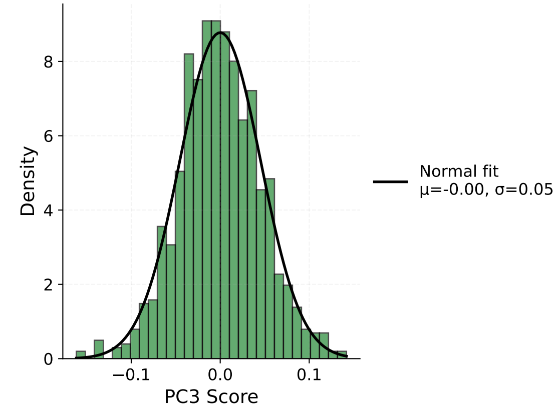
PC3 Distribution
