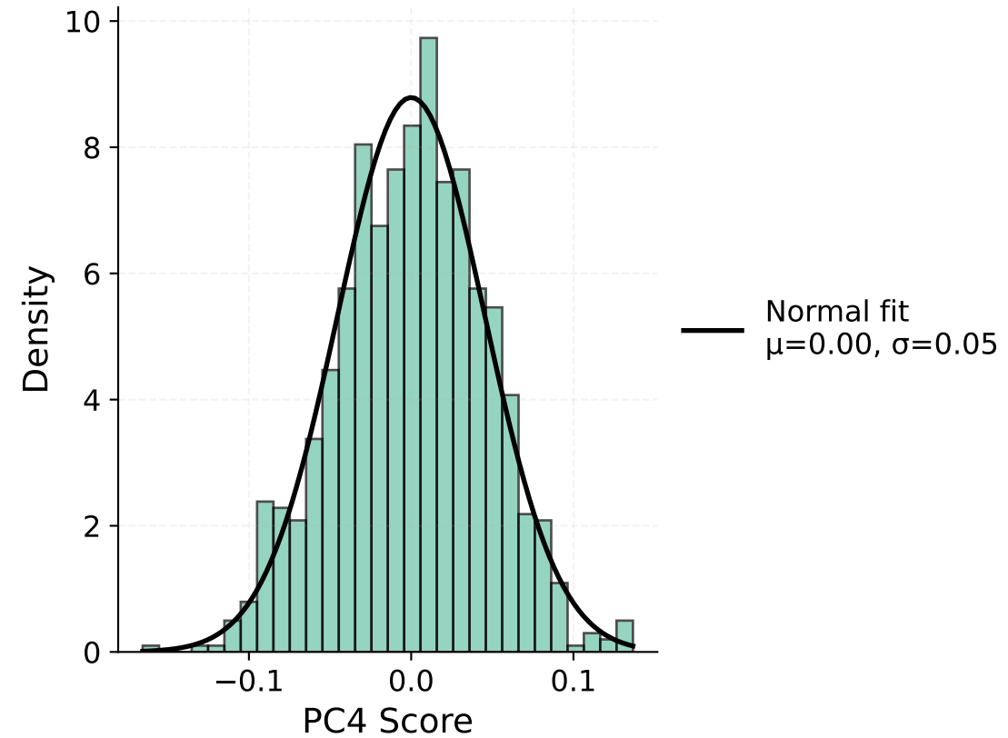
PC4 Distribution
