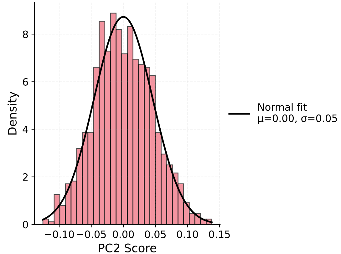
PC2 Distribution
