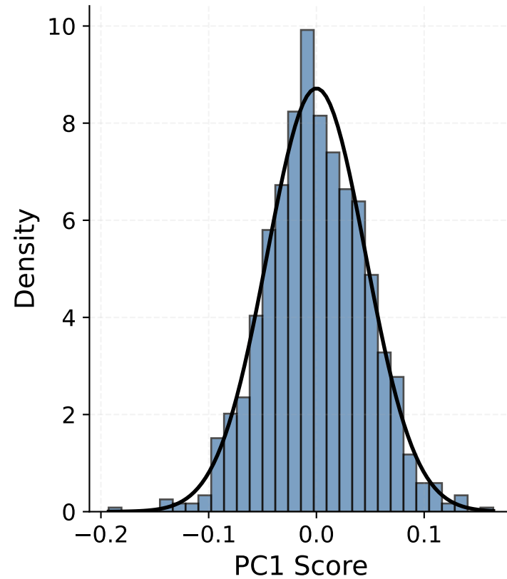
PC1 Distribution
