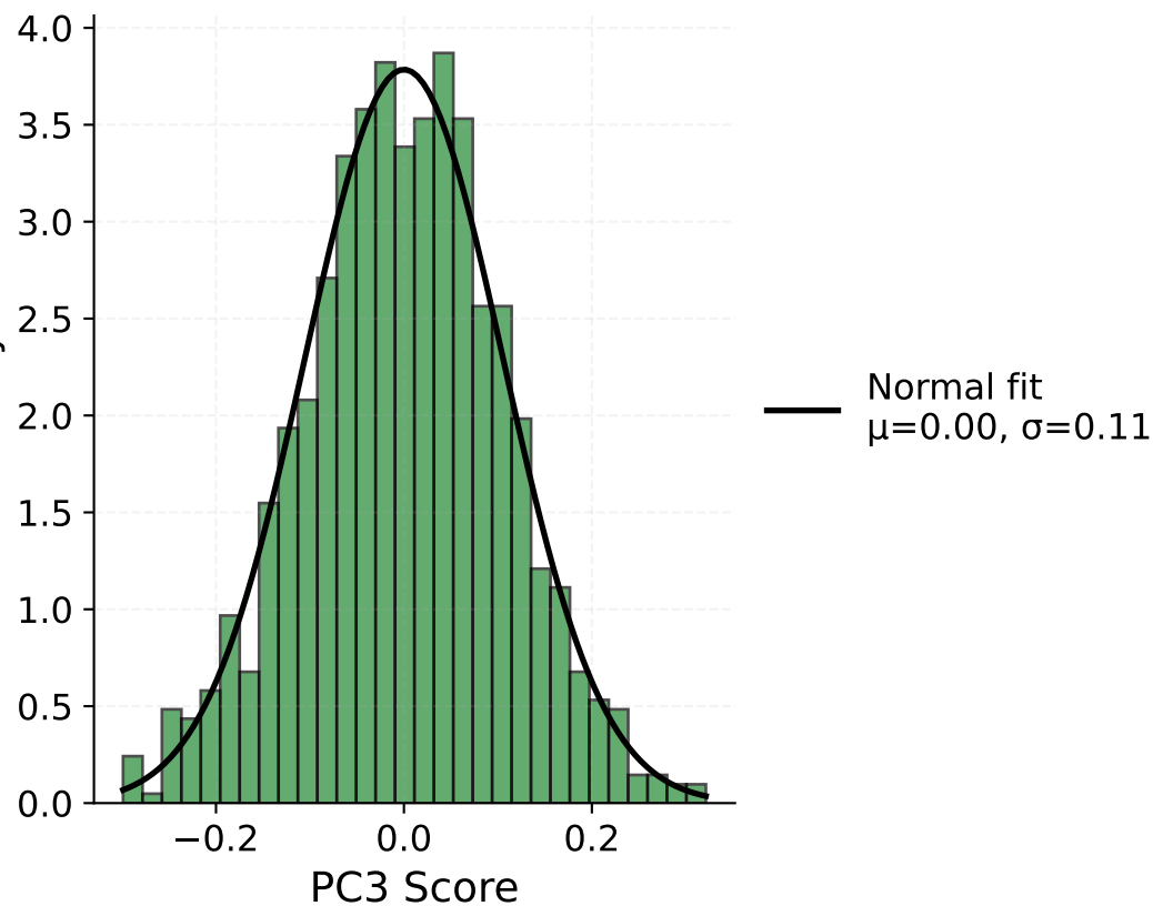
PC3 Distribution
