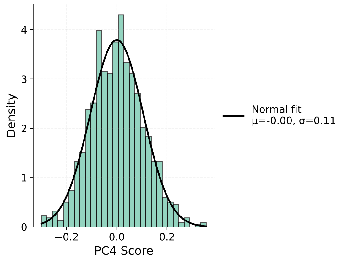
PC4 Distribution
