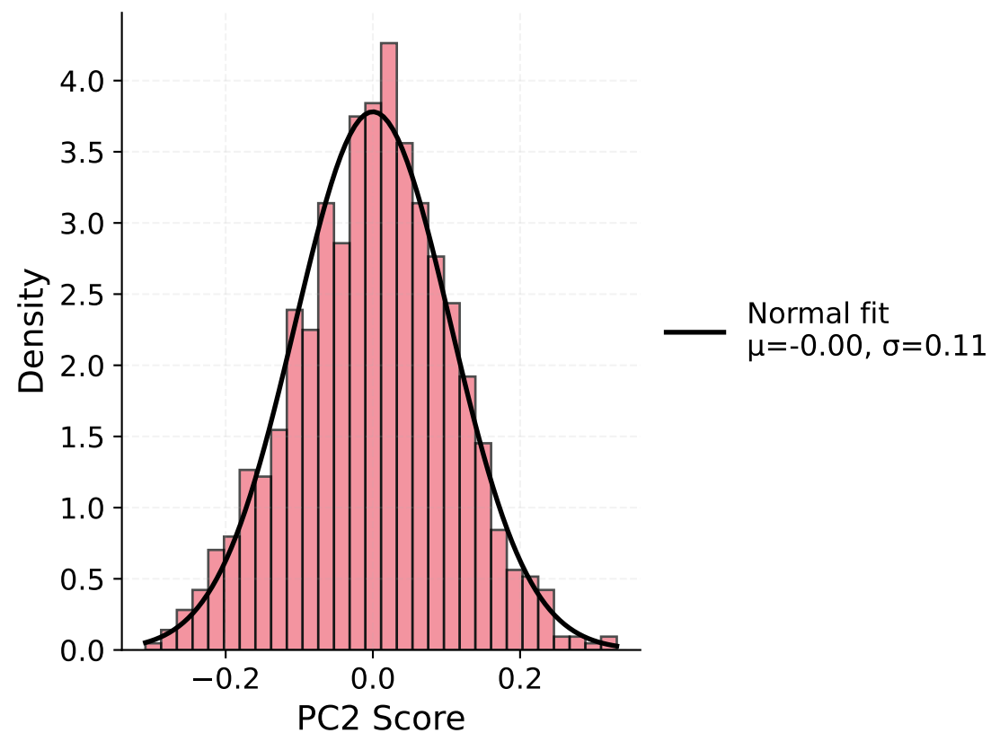
PC2 Distribution
