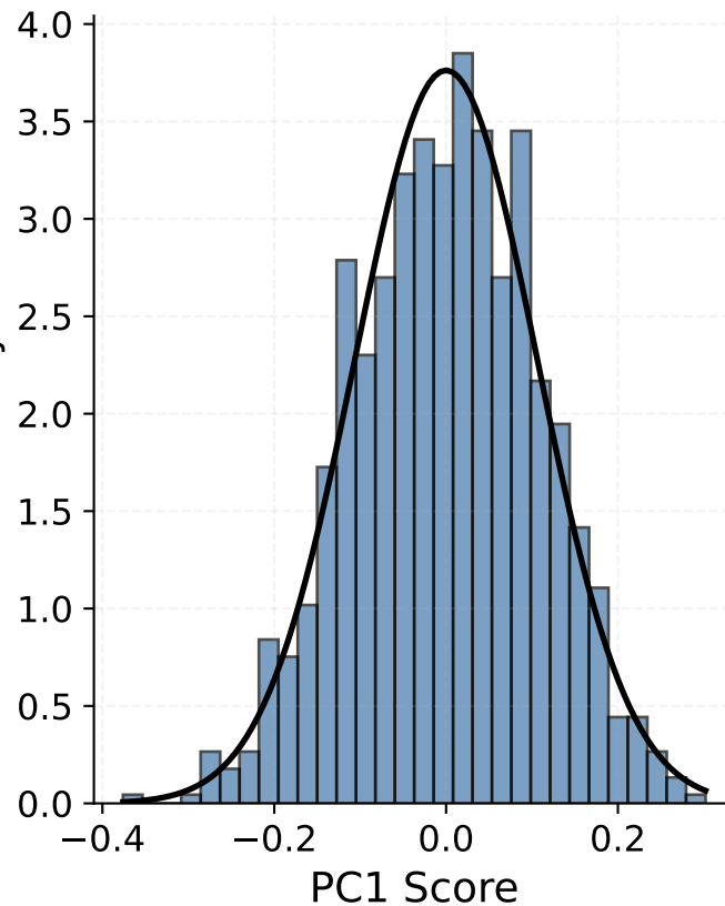
PC1 Distribution
