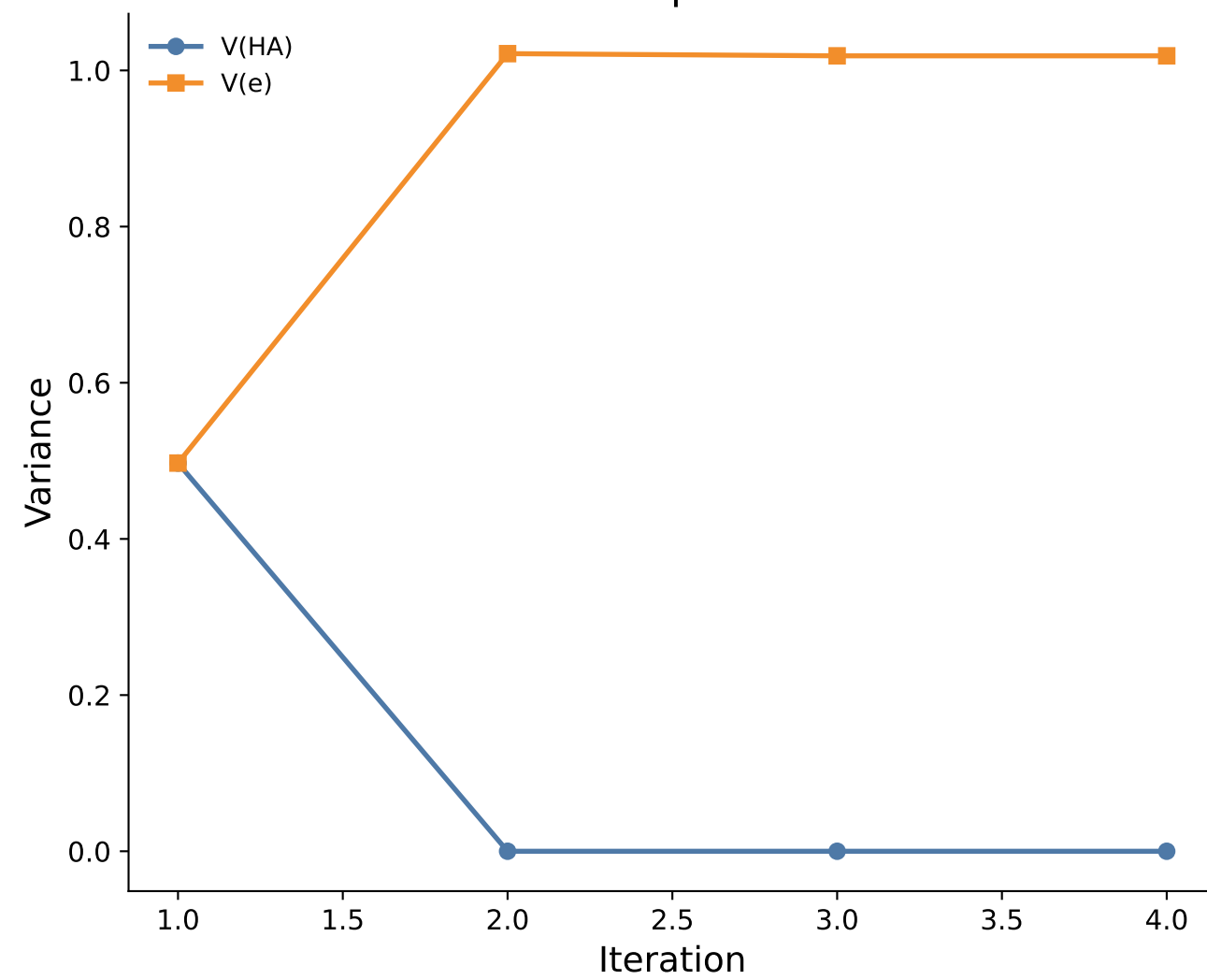
Variance Components Trace
