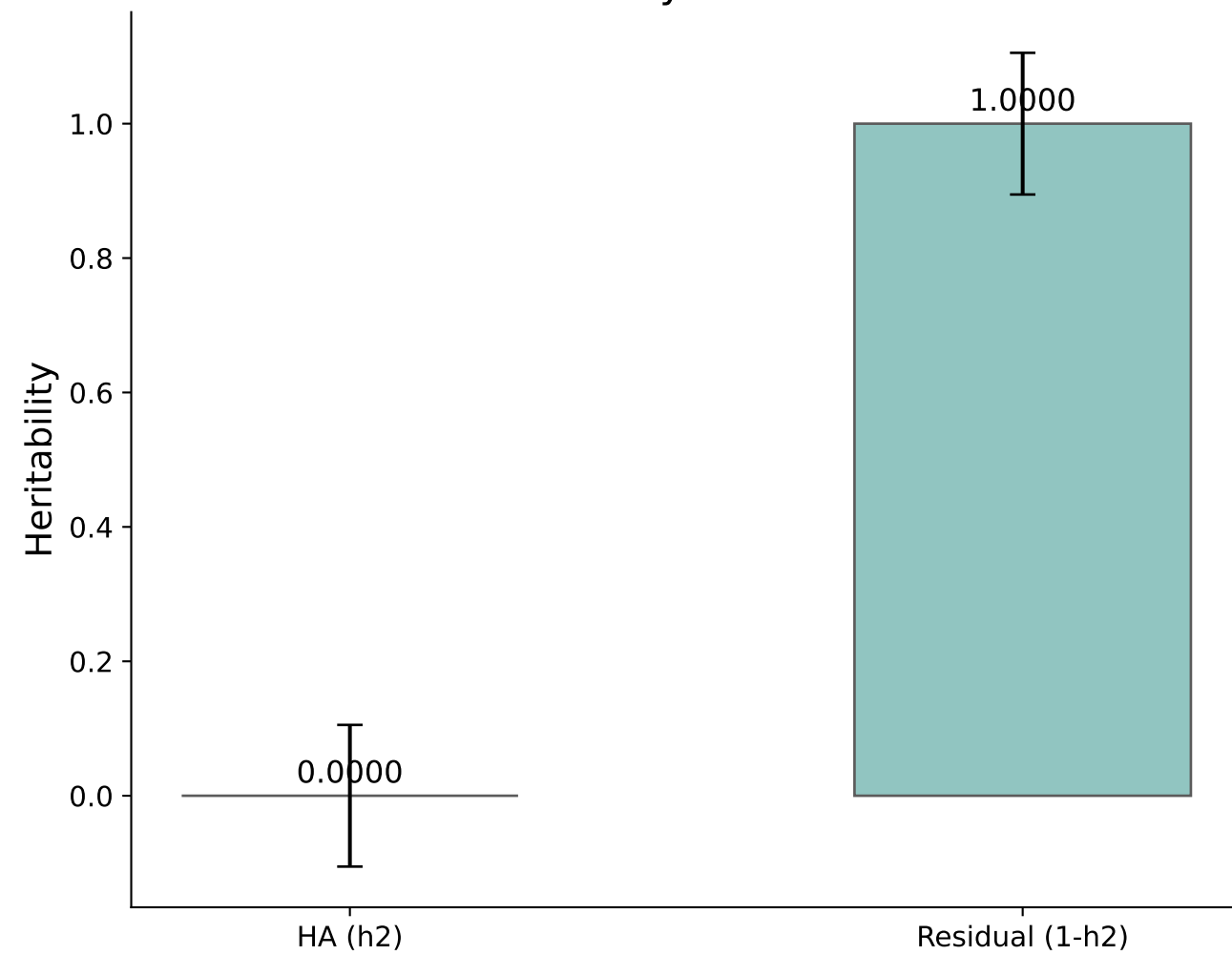
Variance Components Trace
