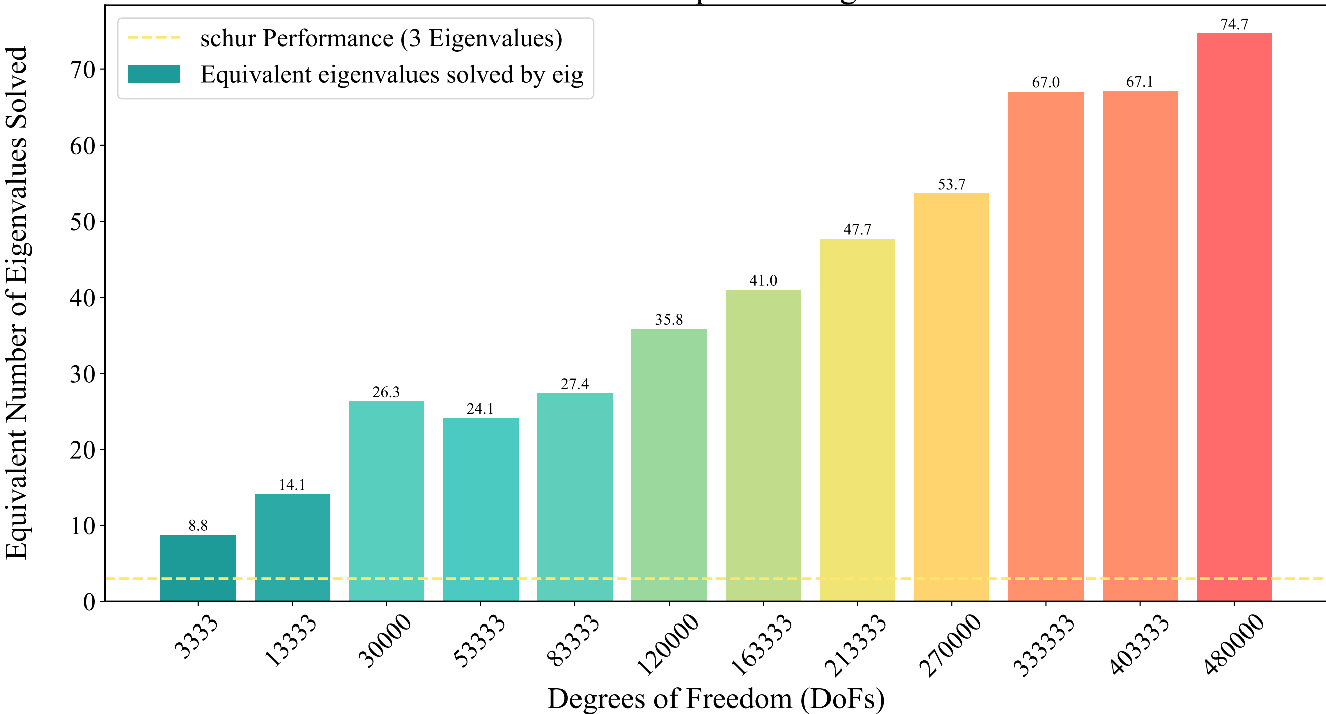
Performance Comparison: eig vs. schur
